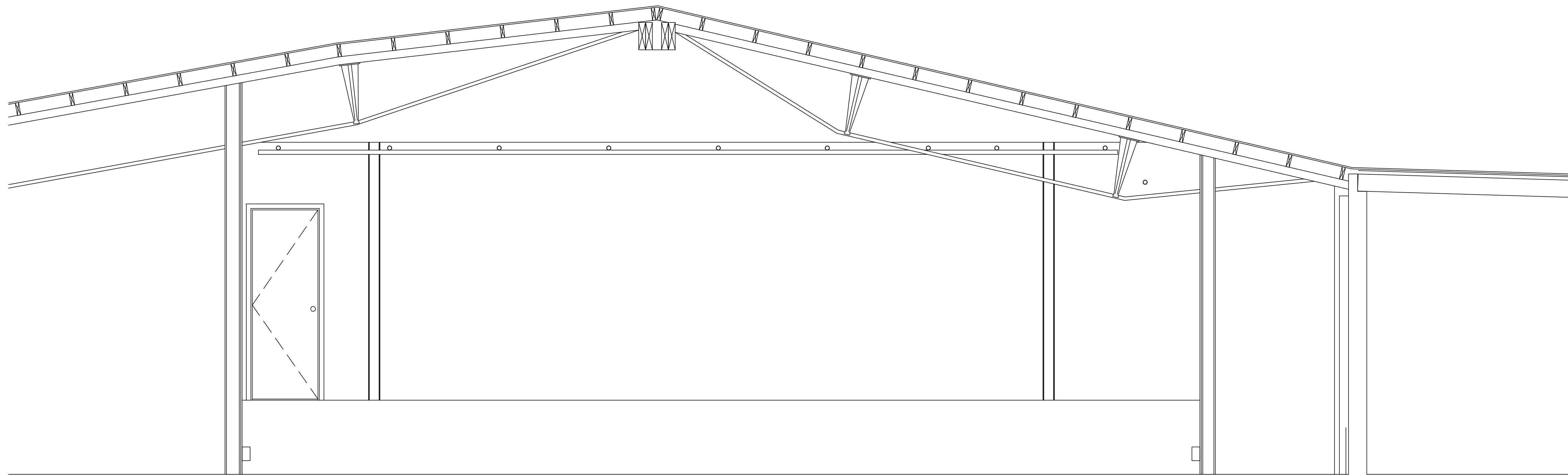
2 Transverse Section
